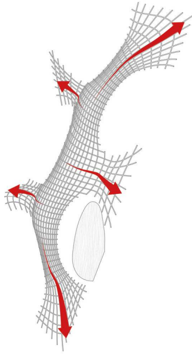
Sharda Library Force Diagram
