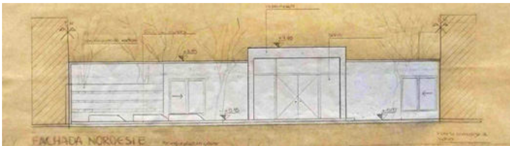
FACHADA PRINCIPAL ESC 1:100
