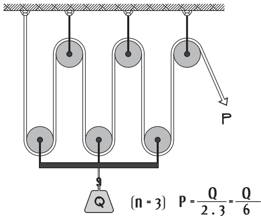
Aparejo Factorial
