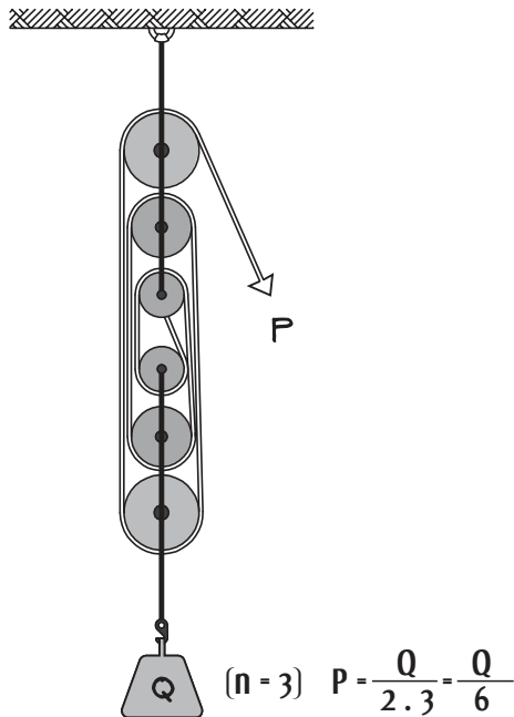
Aparejo Factorial
