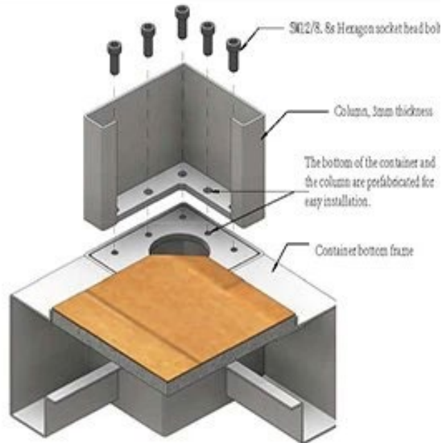
The connection between the column and the bottom of the container-diagram1
