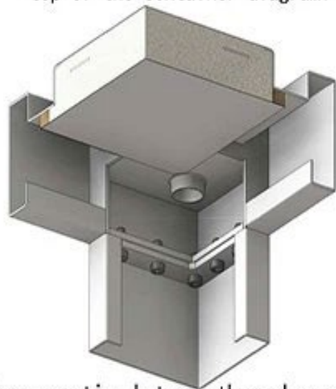
The connection between the column and the top of the container-diagram 2
