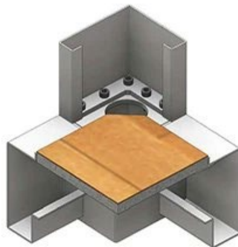
The connection between the column and the bottom of the container-diagram 2
