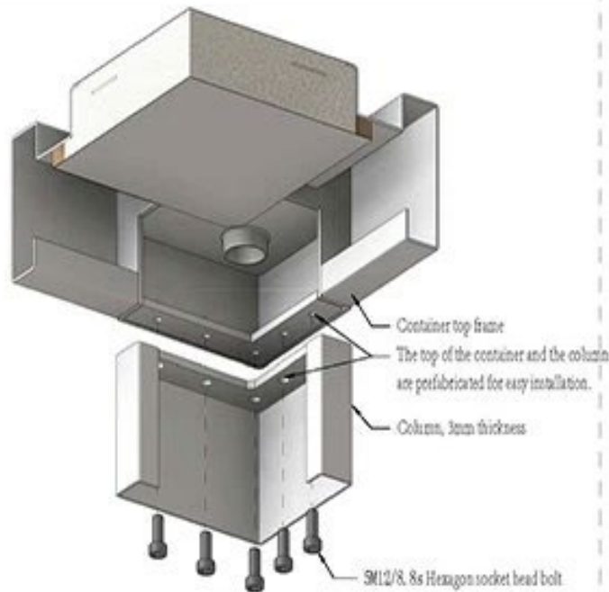
The connection between the column and the top of the container-diagram1
